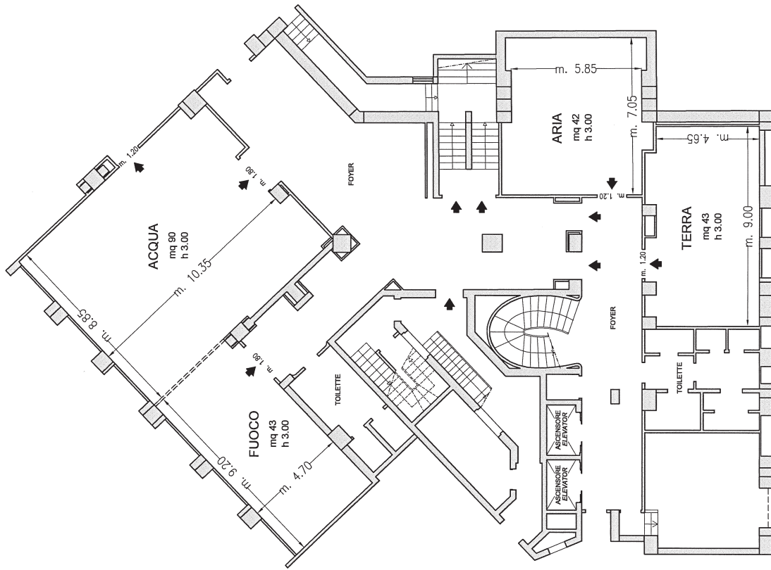
Piano -1 / Basement
