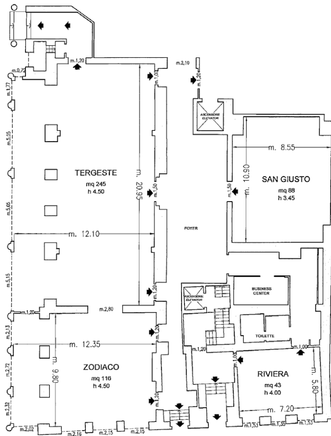
Piano Terra / Ground Floor
