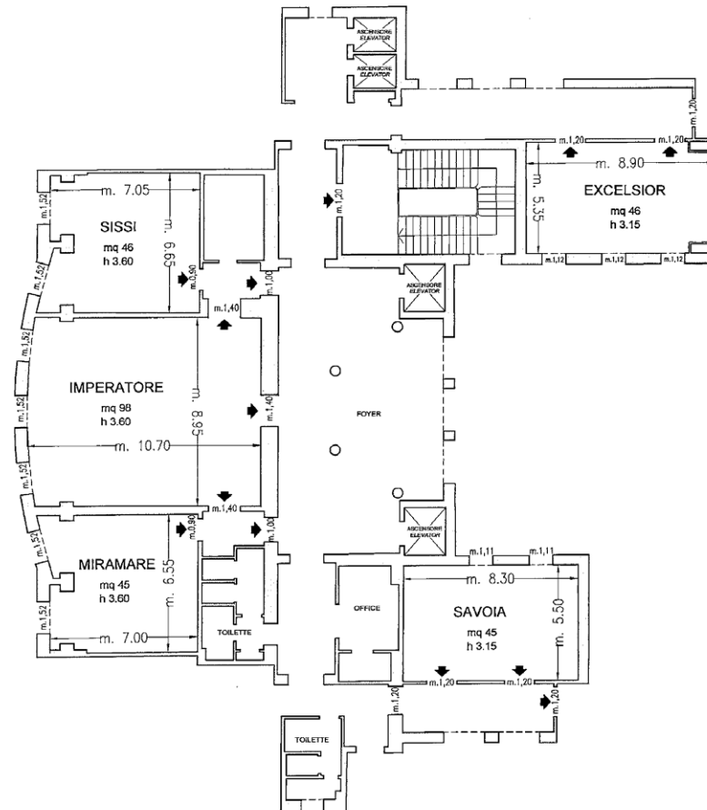
Piano Primo / First Floor
