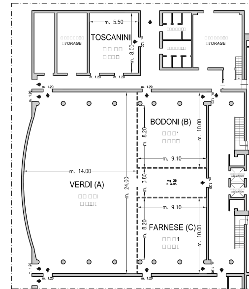
Piano -2 / Floor -2
