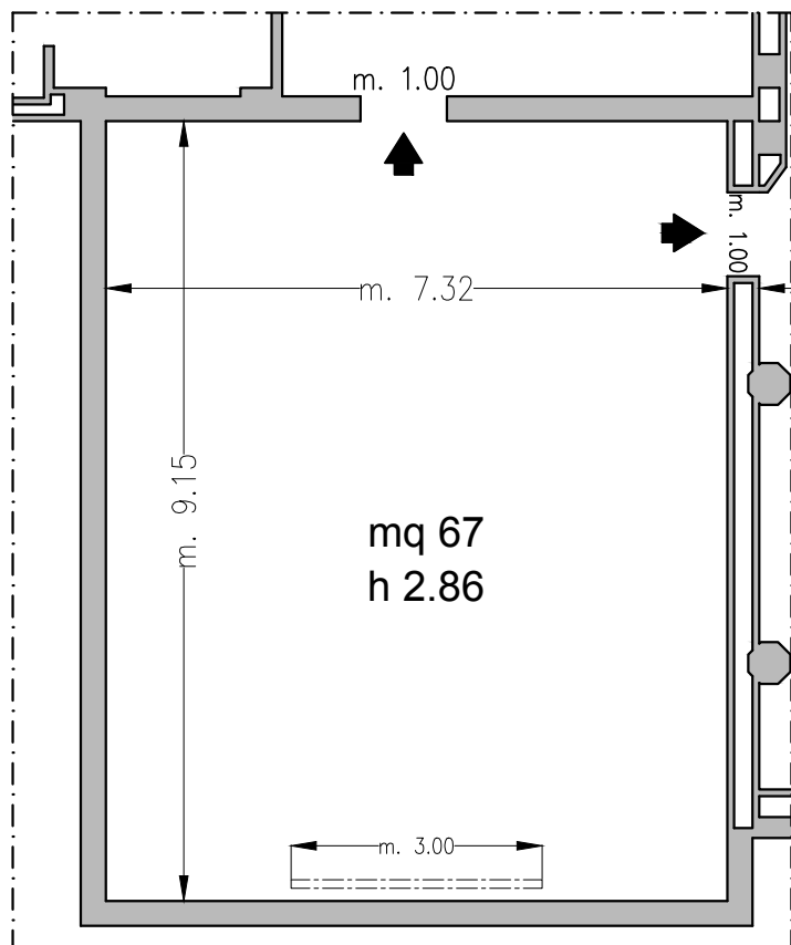
Piano -1 / Basement
