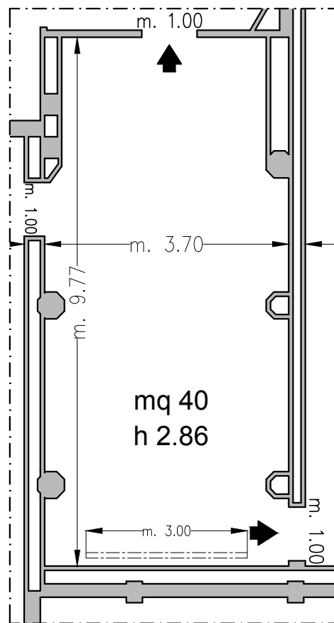
Piano -1 / Basement
