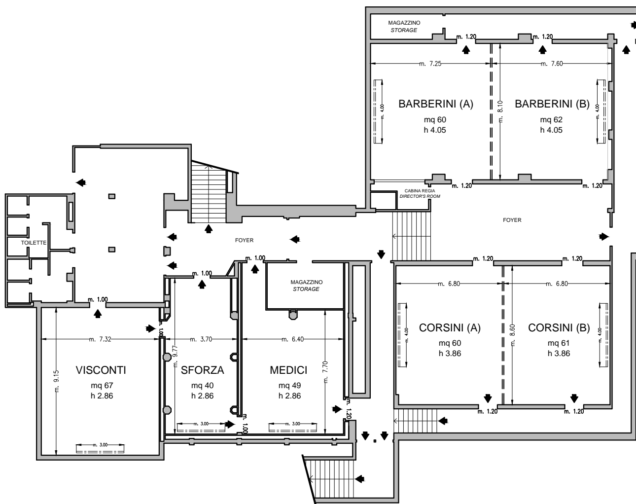
Piano -1 / Basement
