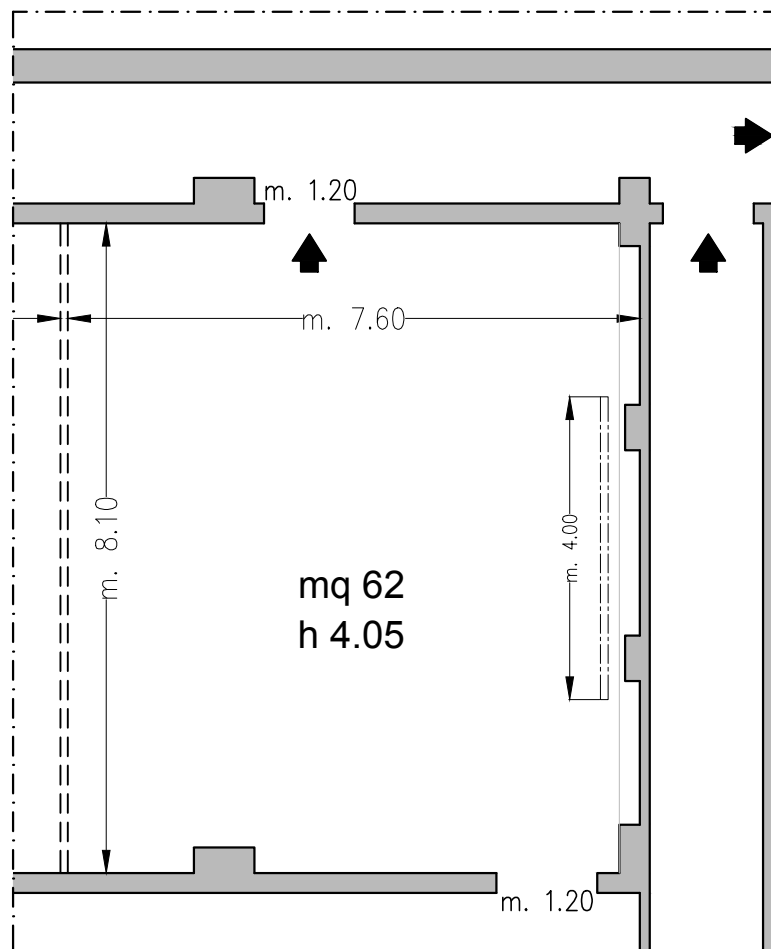
Piano -1 / Basement
