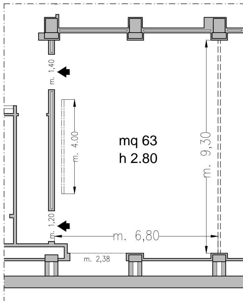
Piano -1 / Basement
