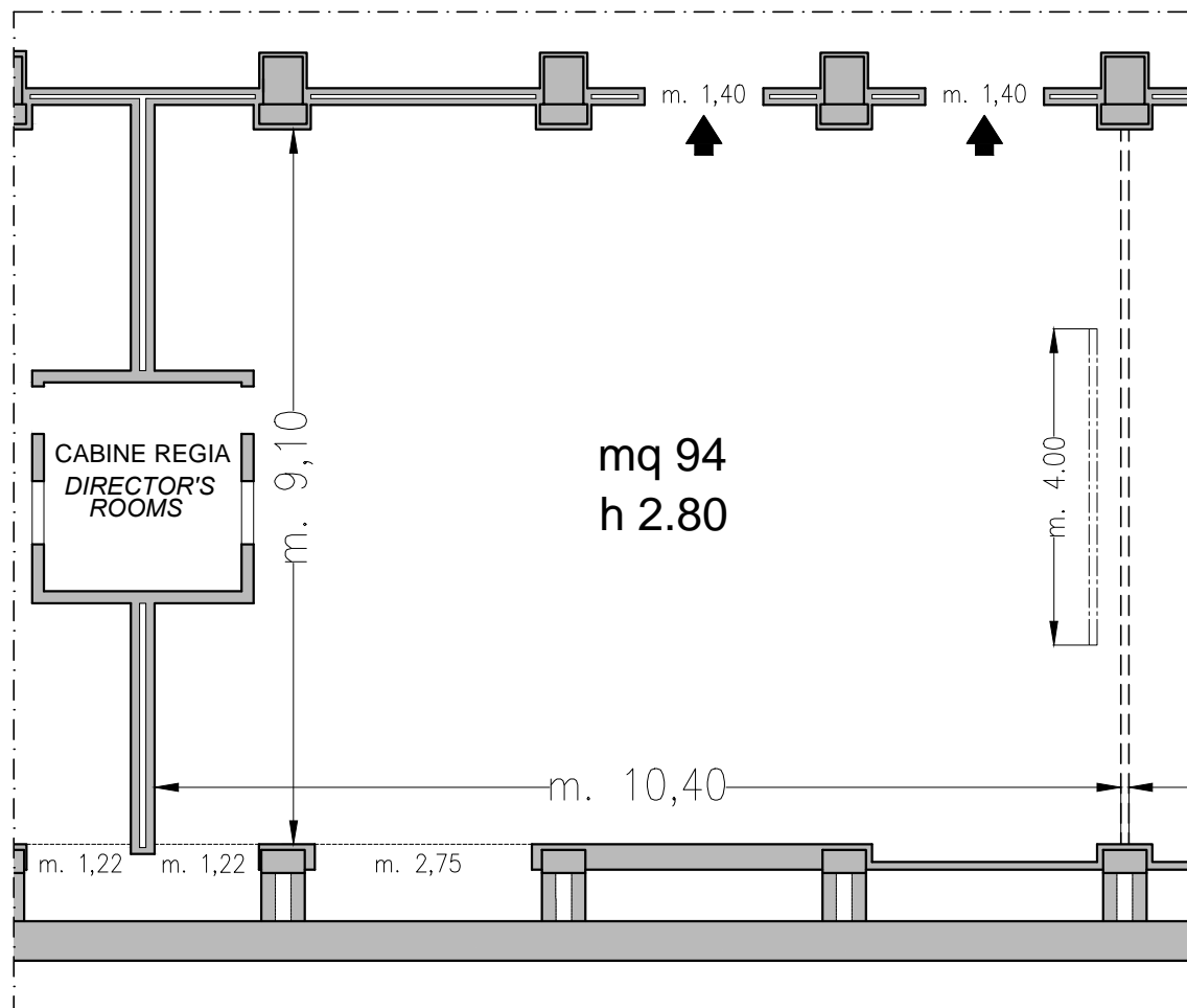
Piano -1 / Basement
