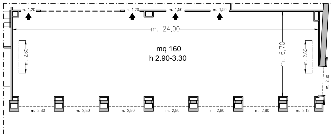
Piano Terra / Ground Floor
