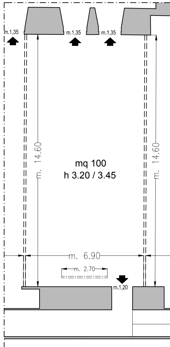
Piano -1 / Basement
