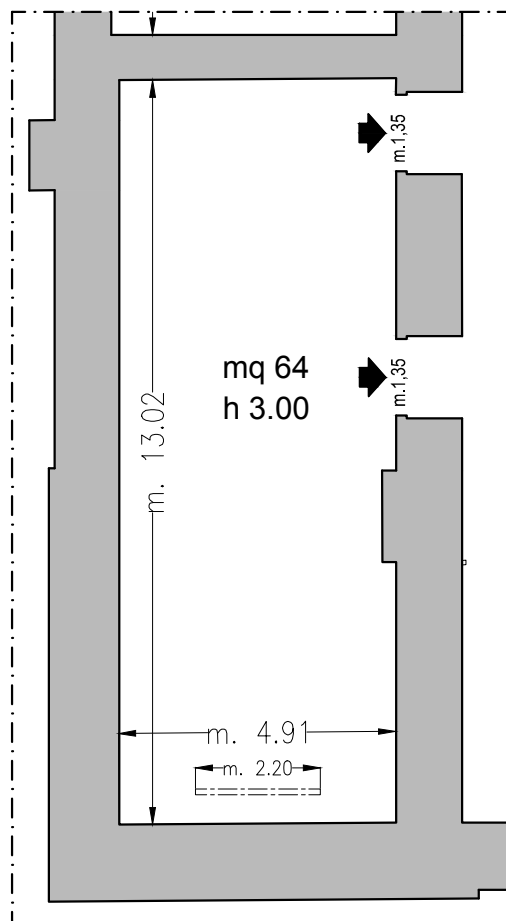
Piano -1 / Basement
