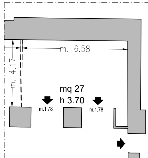
Piano -1 / Basement
