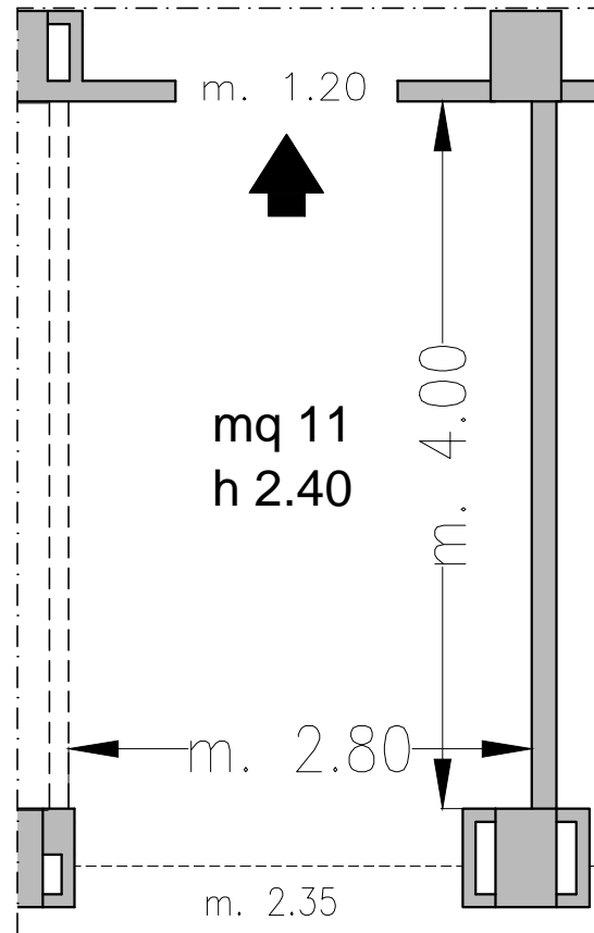
Piano -1 / Basement
