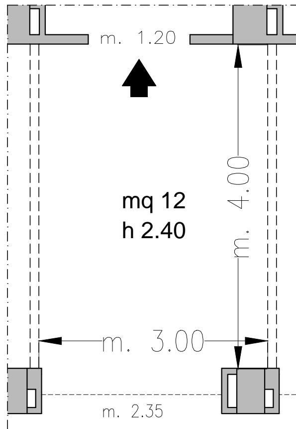
Piano -1 / Basement
