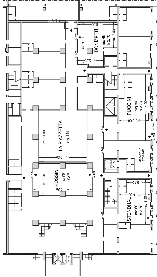
Piano -1 / Basement
