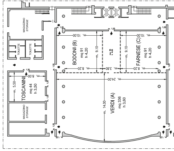
Piano -2 / Floor -2
