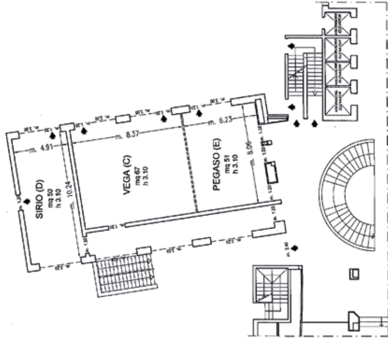
Piano Terra / Ground Floor
