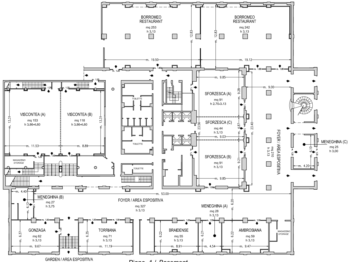
Piano -1 / Basement
