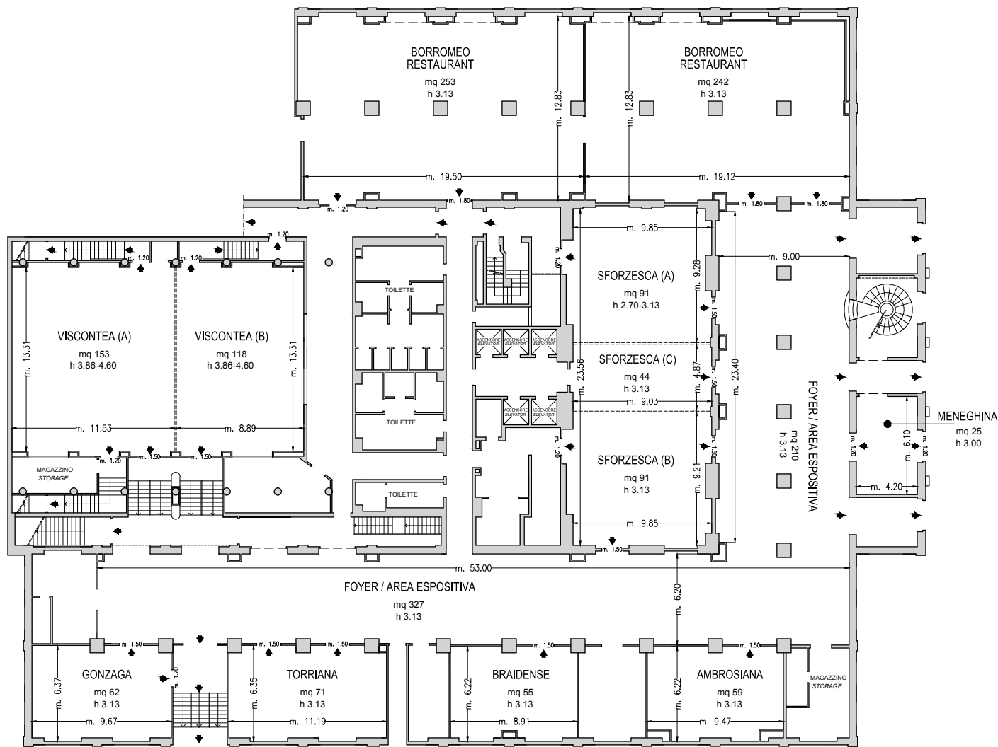
Piano -1 / Basement
